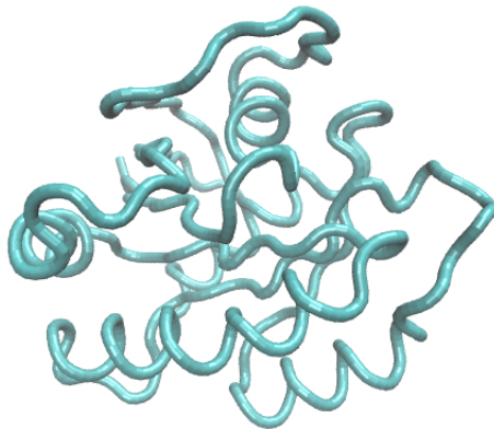
Figure 3: 3D Representation of P21-H-Ras Backbone
